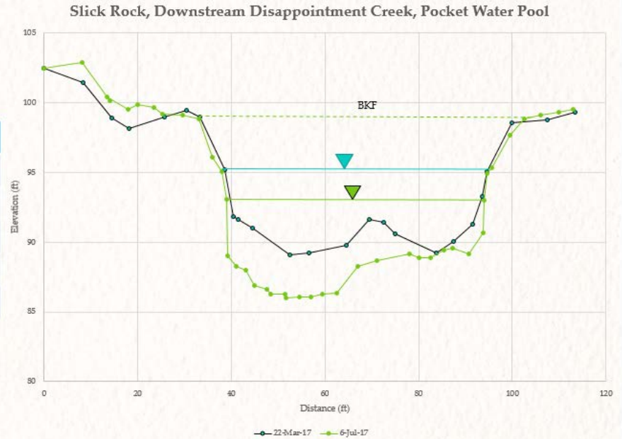
Figure 25. Slickrock Downstream Site, pool cross-sections, pre-release (3/22/17) and post-release (7/6/17). Fairly good scouring occurred, with a decent evacuation of material. Some overall depth was also added. Note the additional deposition on the bank as well.
